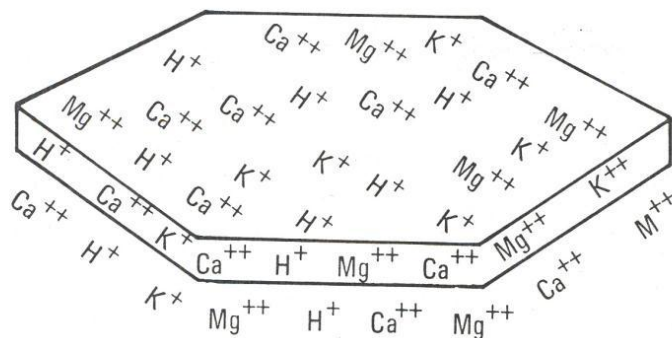
Figure 17.4 — A clay particle with its surface store of negative charges and balancing swarm of adsorped positive ions (cations)
