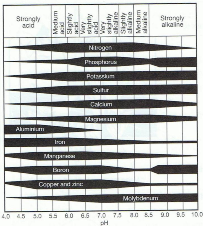
Figure 6. Influence of pH on nutrient availability (Source: Australian Soil Fertility Manual, Third Edition 2006)
